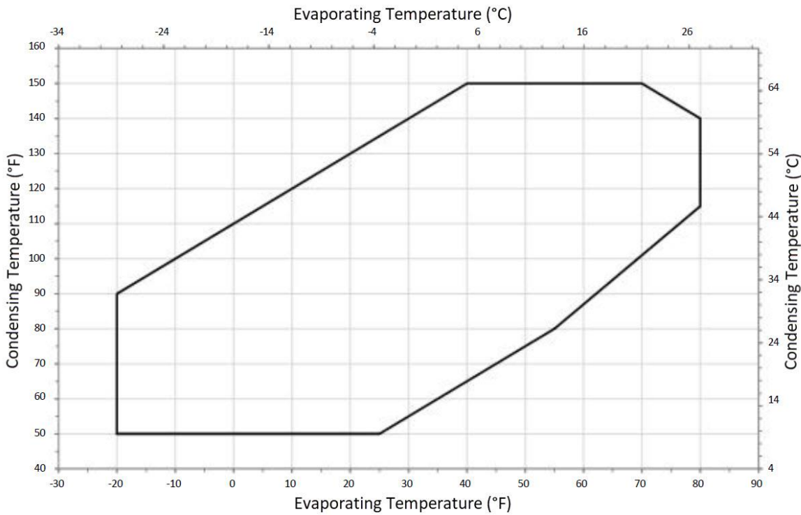
Figure 3 - R-410A 50/60 Hertz Operation
