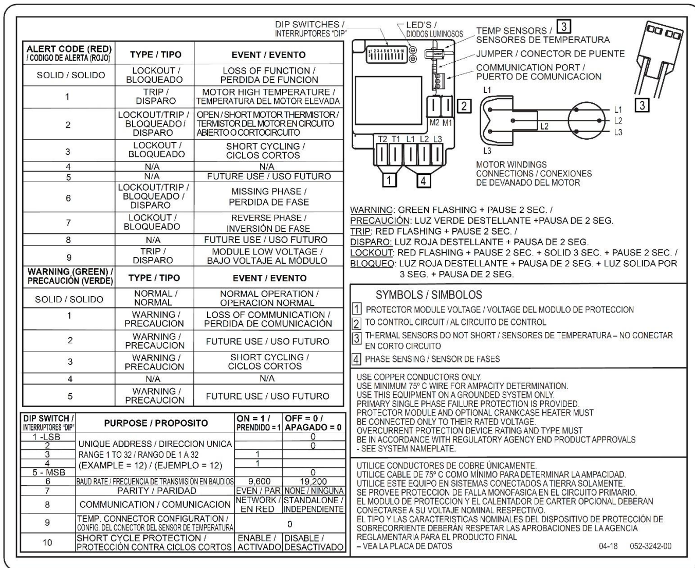
Figure 4 - Compressor Terminal Box Wiring with CoreSense Protection
