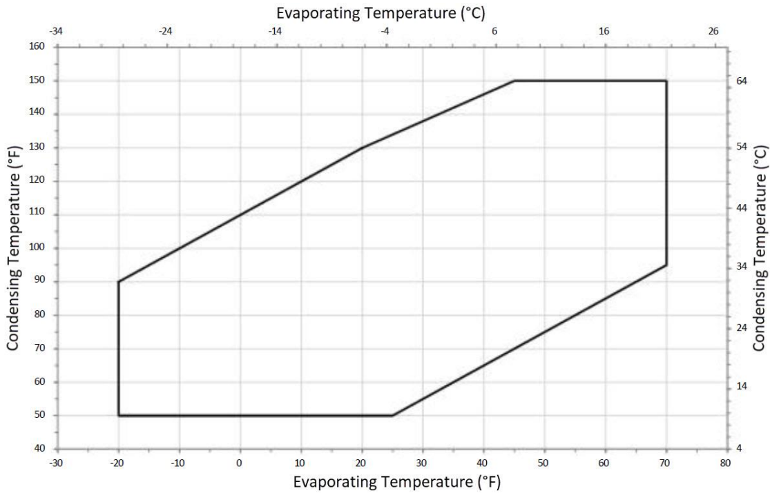
Figure 2 - R-407C, R-22 and R-134a 50/60 Hertz Operation Envelope
