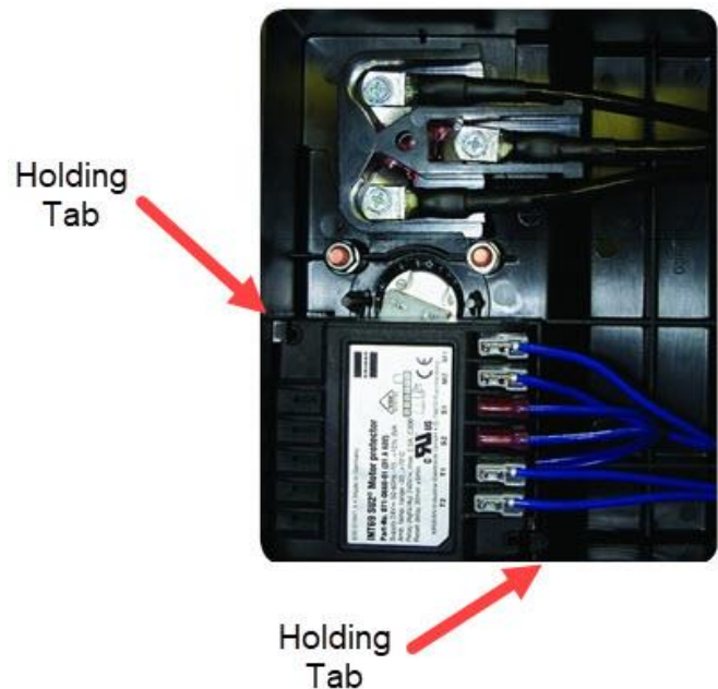
Fig. 1 - Tabs Holding Position
